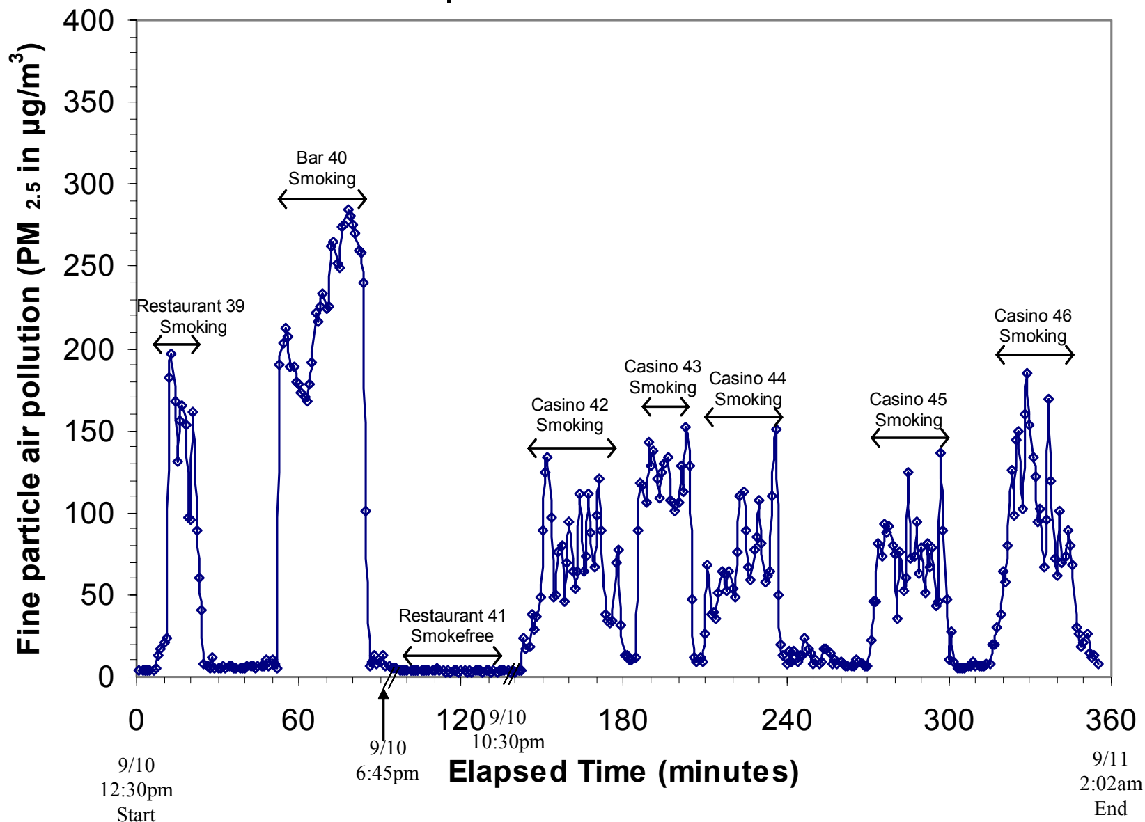
Figure 12 New Jersey Air Monitoring Study September 10 th 2005
